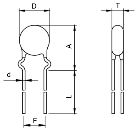
外弯型引线 Outward Crimp Lead
